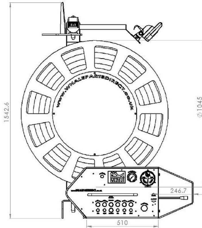
Reel Front View
