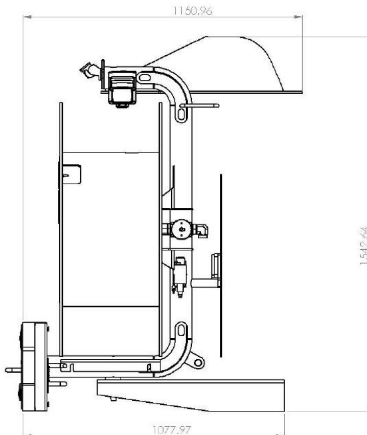
Reel Side View
